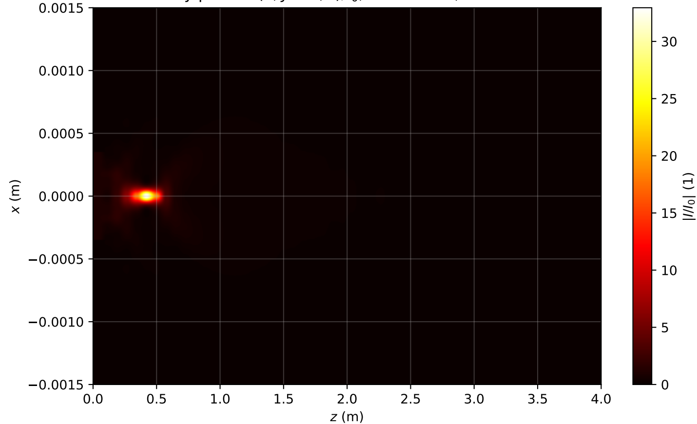
Intensity profile I(x, y = 0, z)/I_0 , P_{in}=2.0P_{cr} , artificial time
